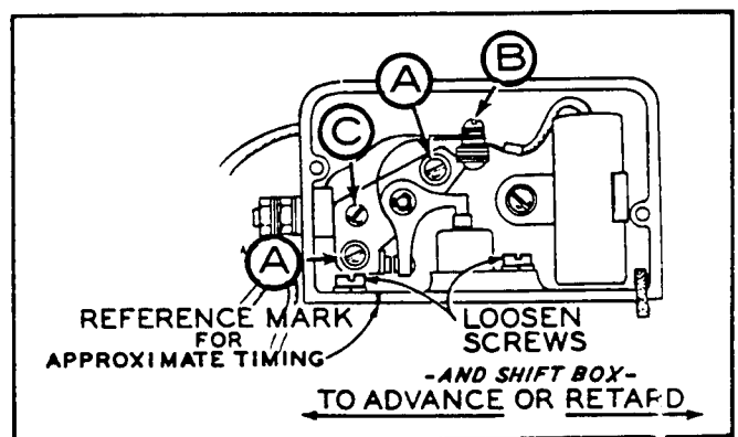
BREAKER POINT ADJUSTMENT
