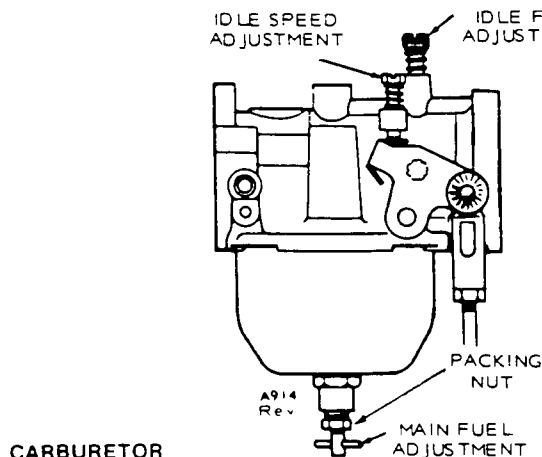
CARBURETOR ADJUSTMENTS
