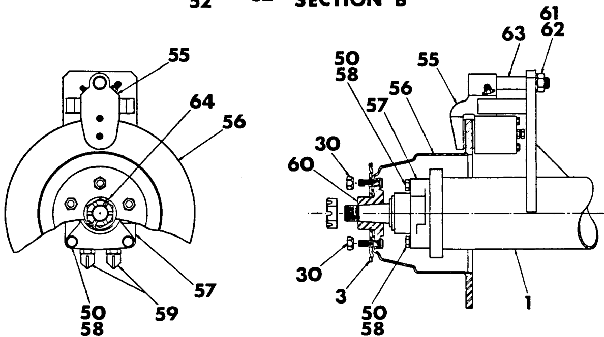
SECTION B
