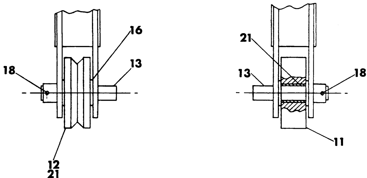
VIEW A
