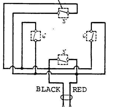
WIRING DIAGRAM
