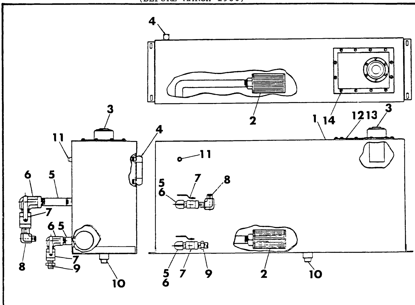
FIGURE 11B.2 - HYDRAULIC TANK ASSEMBLY (RT26E) (RT26G) (RT31E) (RT31G) (SRT31G) (RT40E) (RT40G)
