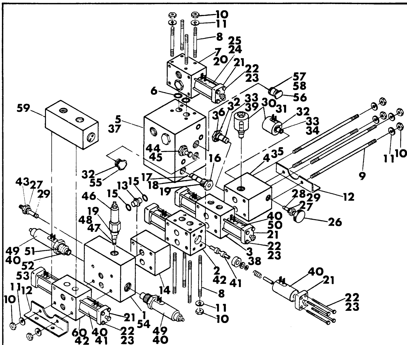
FIGURE 8J - MANIFOLD PACKAGE-WITH OUTRIGGER CONTROL (RT40E) (RT40G)
