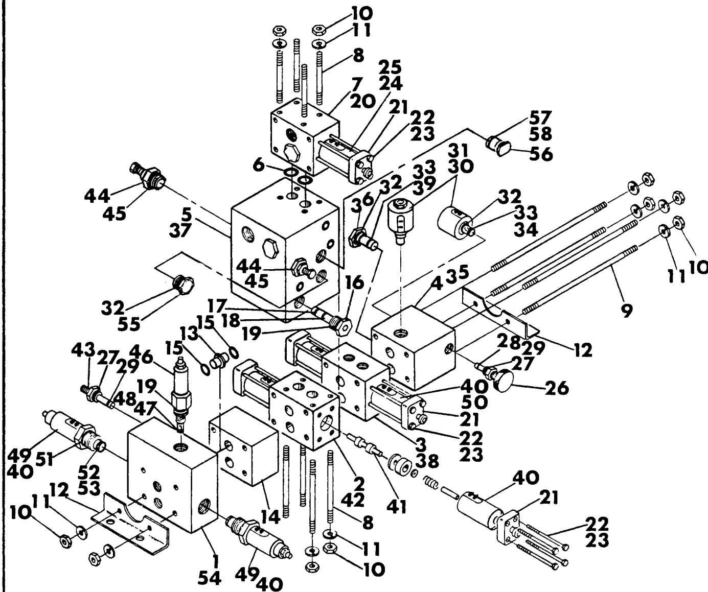
FIGURE 8G - MANIFOLD PACKAGE (RT26E) (RT26G) (RT31E) (RT31G)
