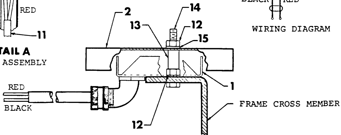
TILT SWITCH INSTALLATION
