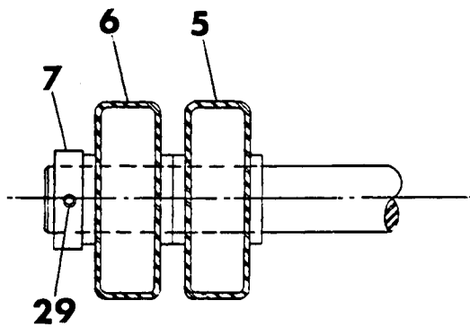
SECTION A
