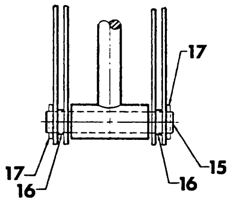
DETAIL B
