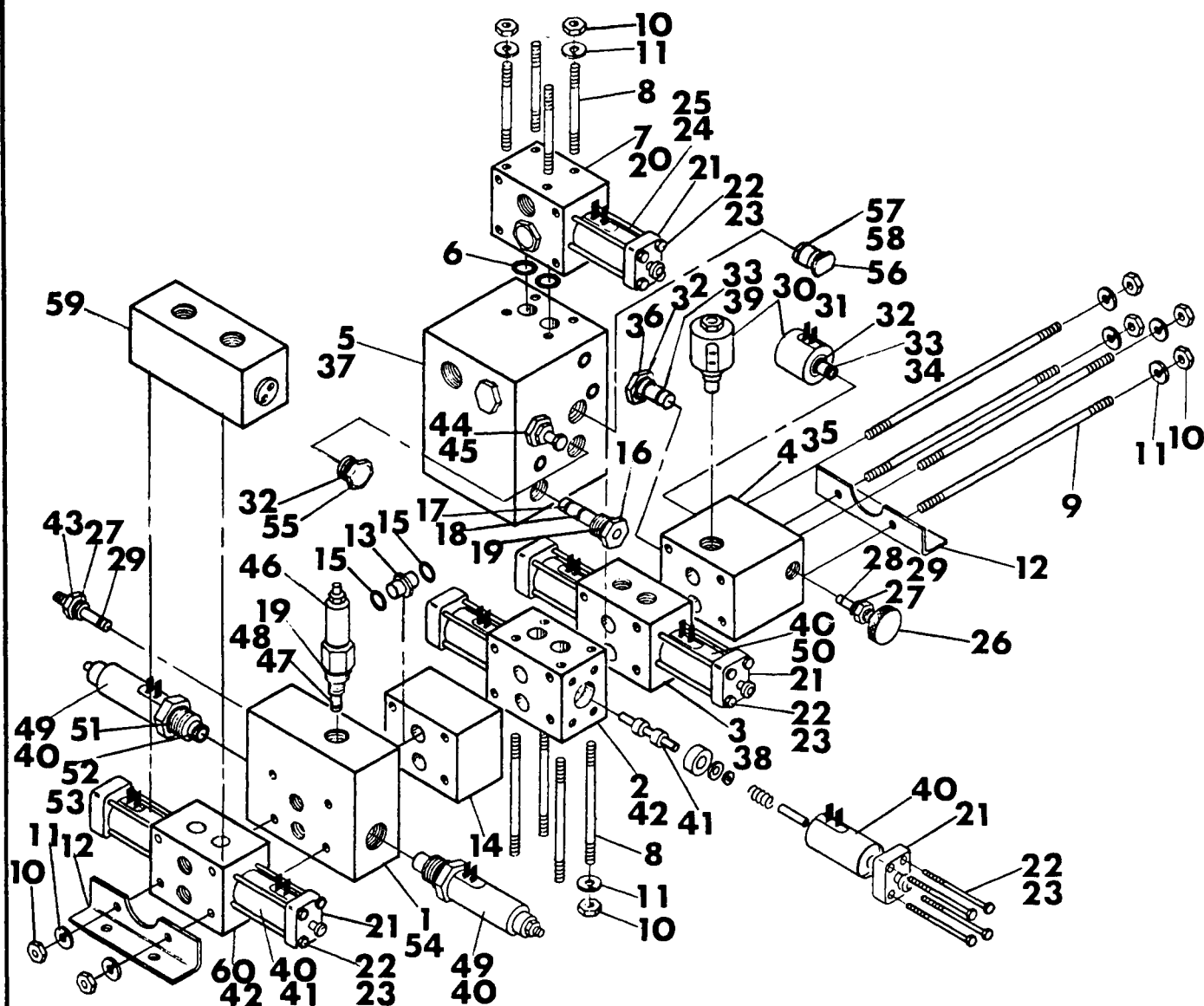
FIGURE 8H - MANIFOLD PACKAGE-WITH OUTRIGGER CONTROL (RT26E) (RT26G) (RT31E) (RT31G) (OPTION)
