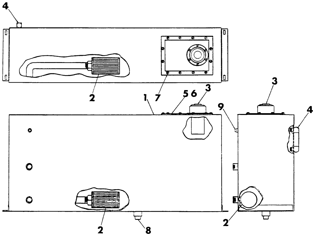
FIGURE 11B - HYDRAULIC TANK ASSEMBLY (RT26E) (RT26G) (RT31E) RT31G) (SRT31G) (RT40E) (RT40G) (BEGINNING MAY 1977 AND STILL BEING USED)
